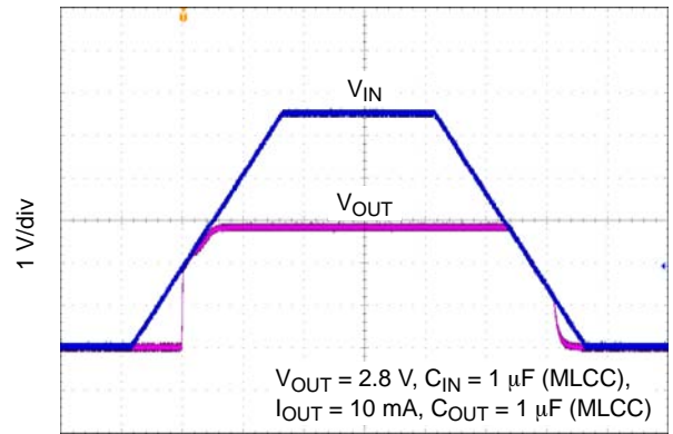
Figure 43. Turn-on/off – Slow Rising V_{IN}
