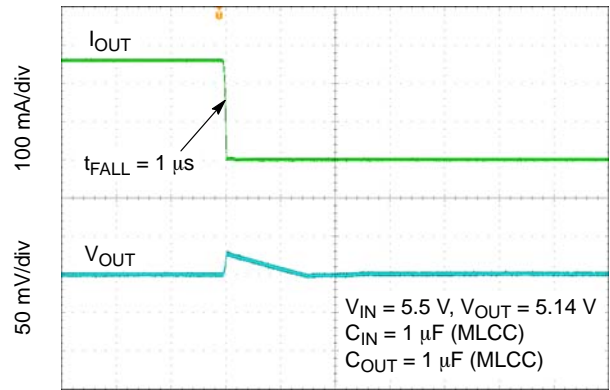
Figure 49. Load Transient Response – 250 mA to 1 mA – V_{OUT} = 5.14\text{ V}
