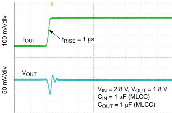
Figure 44. Load Transient Response – 1 mA to 250 mA – V_{OUT} = 1.8 \text{ V}
