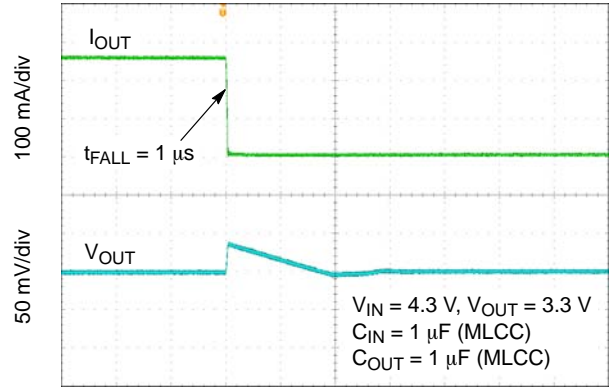
Figure 47. Load Transient Response – 250 mA to 1 mA – V_{OUT} = 3.3\text{ V}
