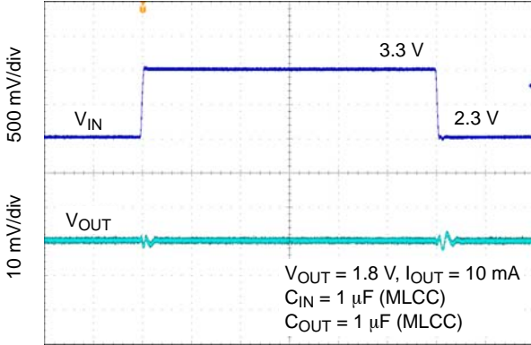
Figure 40. Line Transient Response – V_{OUT} = 1.8 \text{ V}
