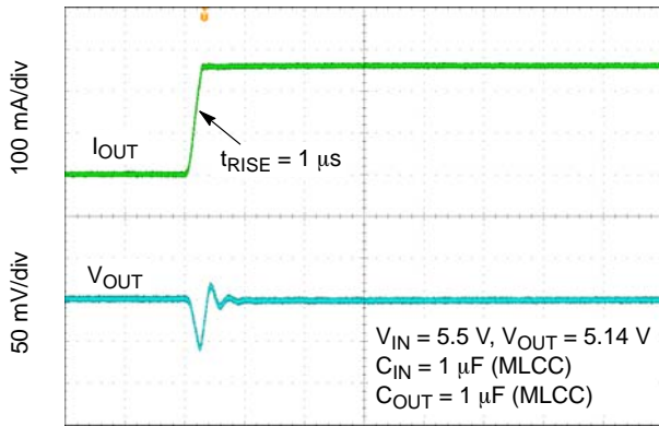
Figure 48. Load Transient Response – 1 mA to 250 mA – V_{OUT} = 5.14\text{ V}
