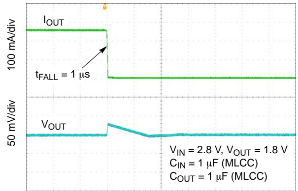
Figure 45. Load Transient Response – 250 mA to 1 mA – V_{OUT} = 1.8 \text{ V}
