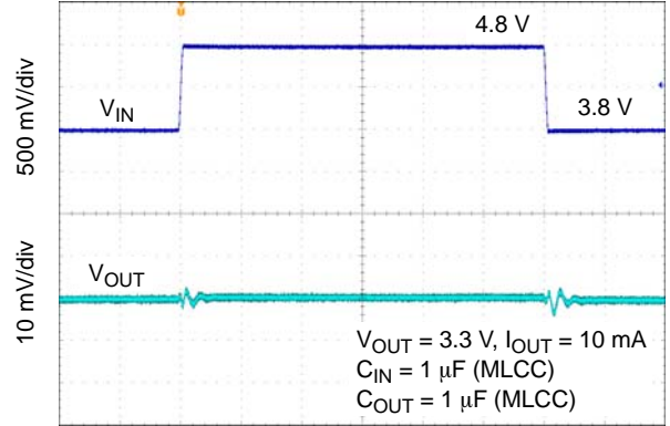
Figure 41. Line Transient Response – V_{OUT} = 3.3 \text{ V}
