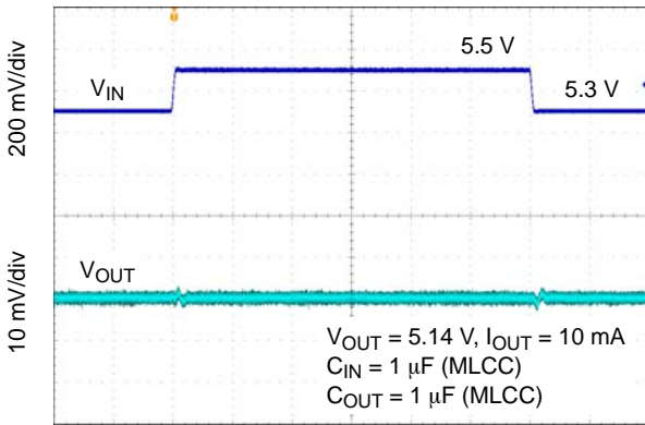
Figure 42. Line Transient Response – V_{OUT} = 5.14 \text{ V}
