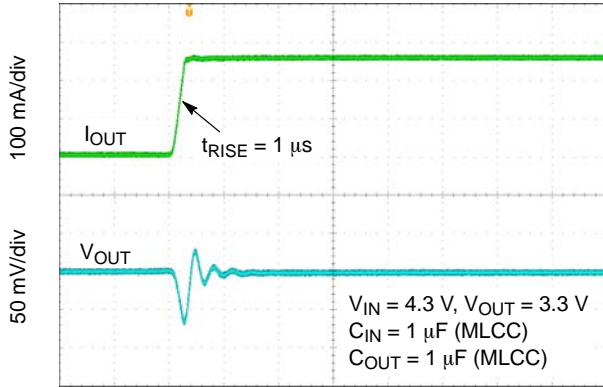
Figure 46. Load Transient Response – 1 mA to 250 mA – V_{OUT} = 3.3\text{ V}
